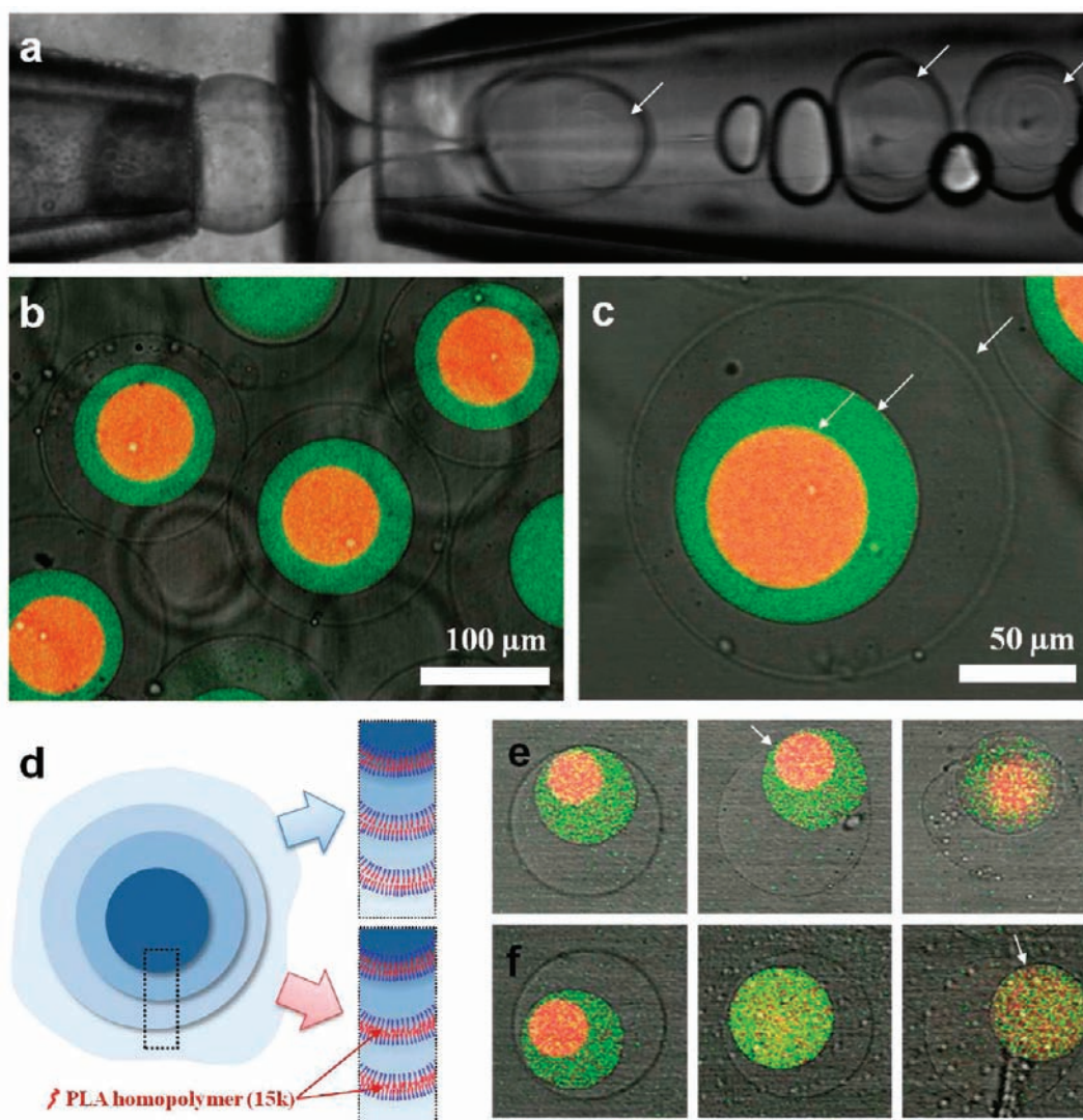
Figure 4. (a) Optical microscope image showing injection of double polymersomes into the innermost drops of double-emulsion drops. (b, c) Confocal microscope images showing triple polymersomes. The arrows denote three membranes of triple polymersomes. (d) Schematic illustration of a triple polymersome showing bilayers with no internal homopolymer on the top right and two of the bilayers containing homopolymer on the bottom right. (e) Series of confocal images showing sequential dissociation of membranes from the outermost to the middle of triple polymersome, consisting of a PLA-homopolymer-free bilayer for all three membranes, in a mixture of water and ethanol in a volume ratio of 1:1. (f) Series of confocal images showing sequential dissociation of membranes from the innermost to the outermost of triple polymersomes, consisting of a PLA-homopolymer-free bilayer for the innermost membrane and a PLA-homopolymer-loaded bilayer for the middle and outermost membranes, in the same mixture of water and ethanol.
