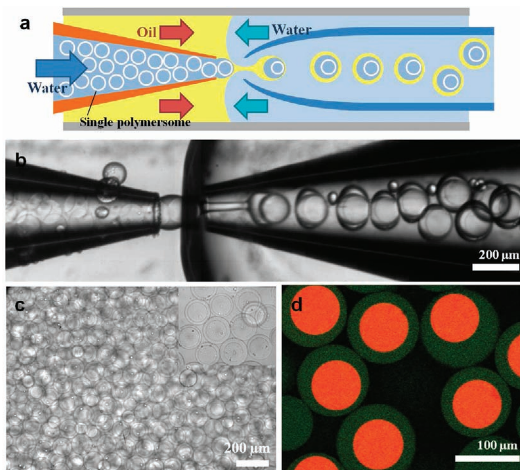
Figure 1. (a) Schematic illustration of the microfluidic device for preparation of double polymersomes containing a single inner polymersome. (b) Optical microscope image showing injection of polymersomes into the innermost drops of double-emulsion drops, where the breakup of middle phase is triggered by the polymersomes. (c) Optical microscope and (d) confocal microscope images of double polymersomes containing a single inner polymersome. Inset of (c) shows a diluted suspension of double polymersomes.
