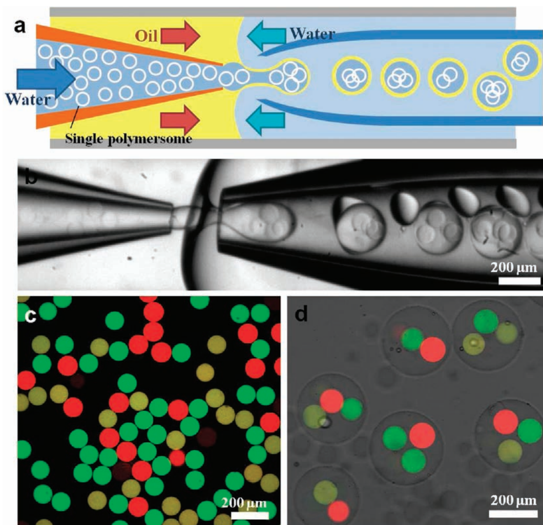
Figure 2. (a) Schematic illustration of the microfluidic device for preparation of double polymersomes containing several inner polymersomes. (b) Optical microscope image showing injection of polymersomes into the innermost drops of double-emulsion drops, where the breakup of the middle phase is triggered by the core drops of the aqueous suspension. (c) Confocal microscope image of a mixture of monodisperse single polymersomes encapsulating a red dye, a green dye, and a mixture of red and green dyes, respectively. (d) Confocal microscope image of double polymersomes containing several inner polymersomes with three different colors.
